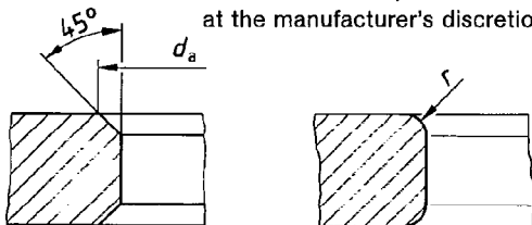
Detail X
